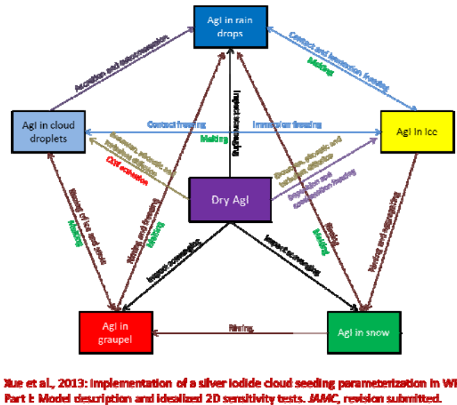
Figure 1: Implementation of a silver iodide cloud seeding module in the WRF Model.
