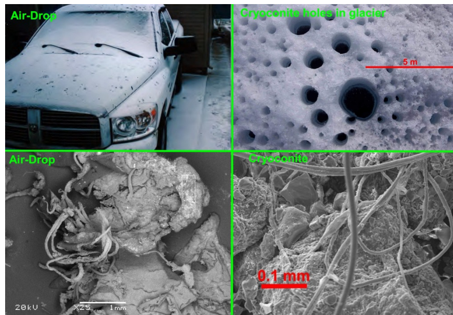
Figure 5. From [48]. Upper Left: Air-Drop Distribution; Upper Right: Cryoconite-hole Distribution in Glacier; Lower Left: Air-Drop Synthetic Cryoconite; Lower Right: Natural Cryoconite
