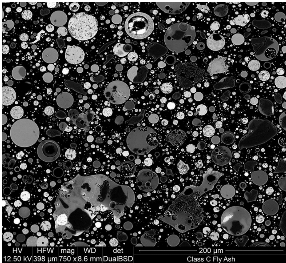
Figure 4. From [16]. Polished section of coal fly ash embedded in epoxy
