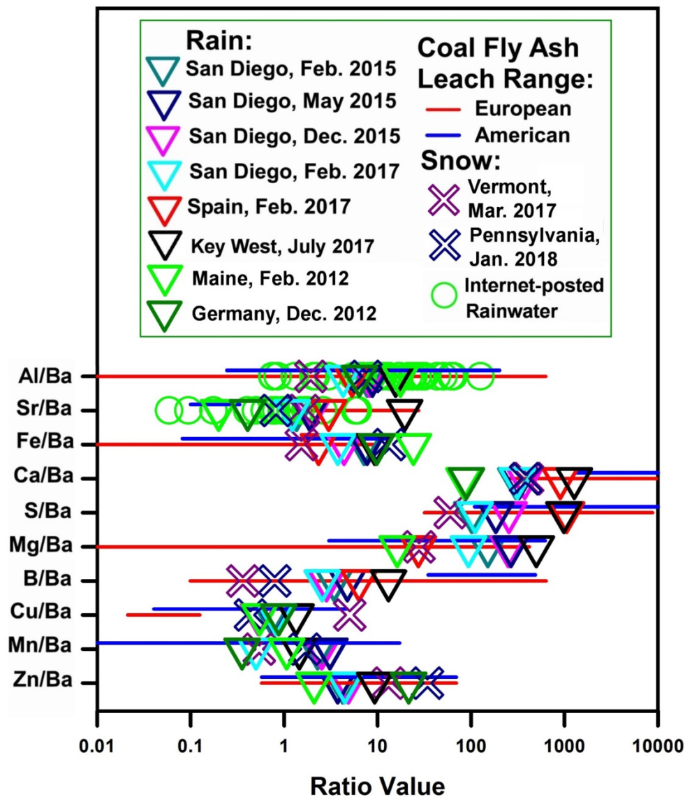
Figure 2. From [26], showing the similarity of element ratios measured in rainwater and snow with the range of comparable element ratios measured in the laboratory lixiviate of water-leach experiments [22, 27]
