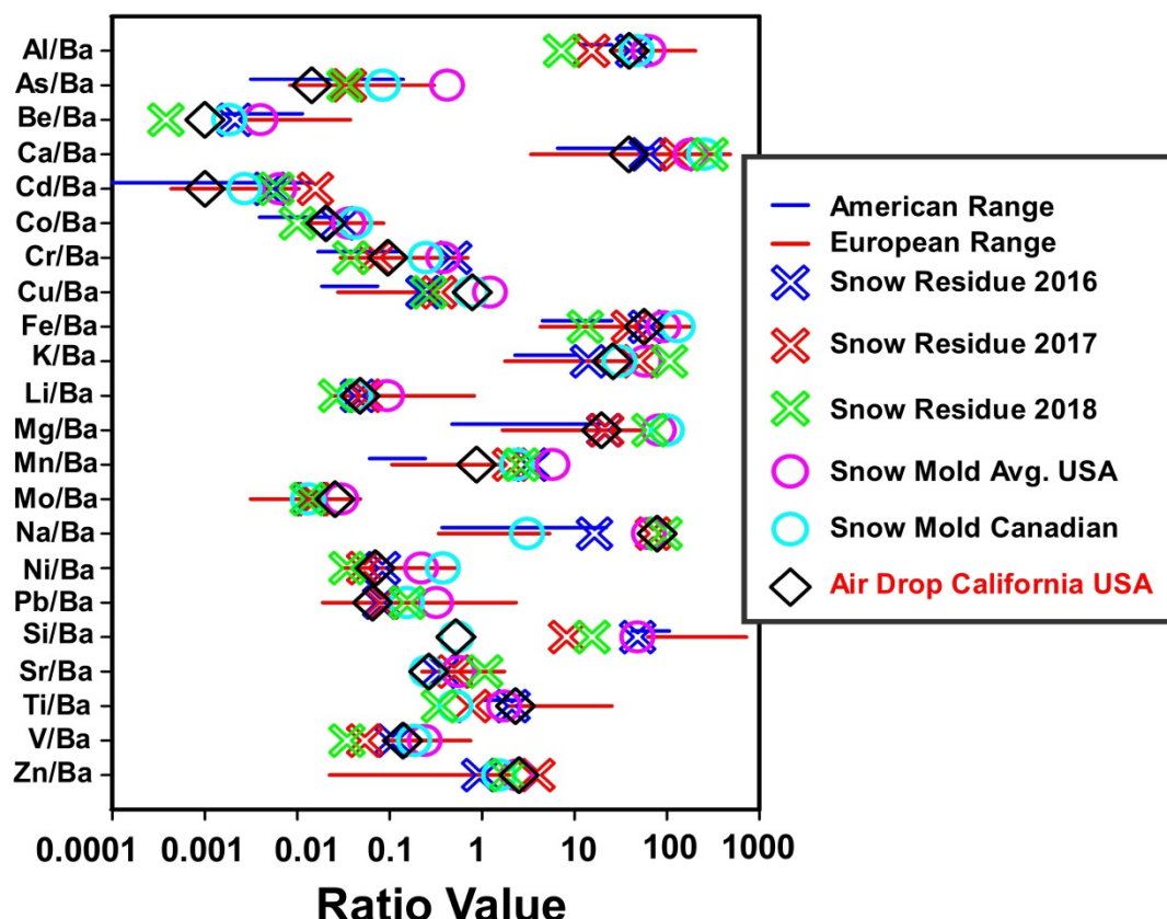
Figure 3. From [28], comparison of analytical results with the ranges of European [22] and American [27] coal fly ash samples
