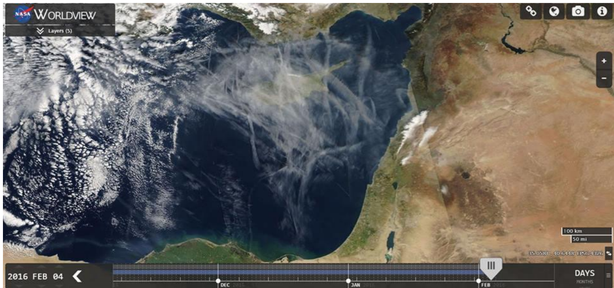
Figure 5. NASA Worldview satellite image from February 4, 2016 showing jet-laid trails blanketing the air above the Republic of Cyprus but nearly absent in surrounding regions.
