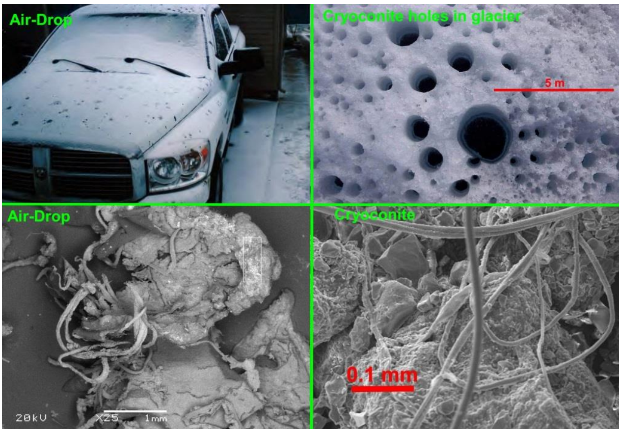
Figure 3. Upper Left: Air-Drop Distribution; Upper Right: Cryoconite-hole Distribution in Glacier; Lower Left: Air-Drop Artificial Cryoconite; Lower Right: Natural Cryoconite.
