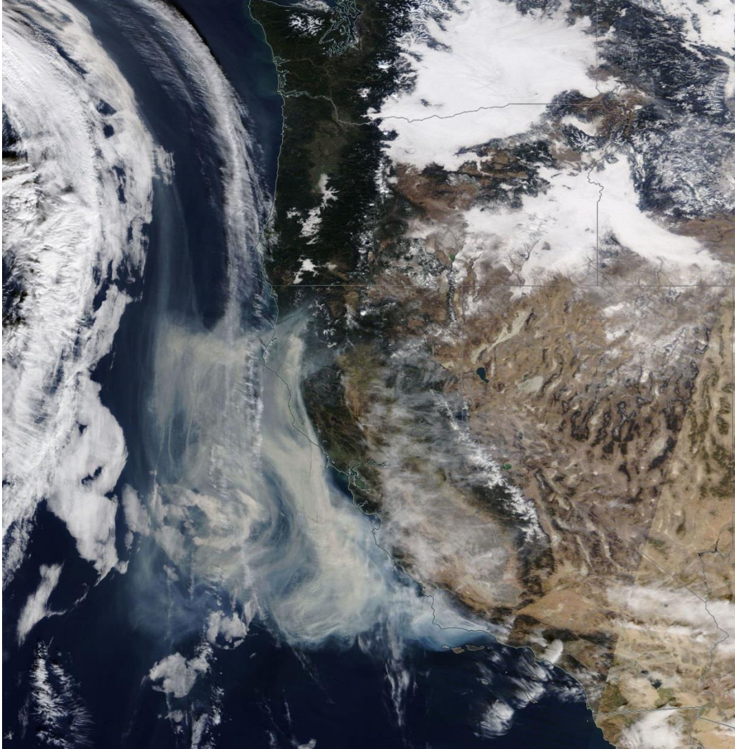
Figure 4. NASA Worldview of the California coast on December 11, 2017.
